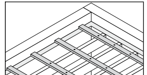
Flat roof
