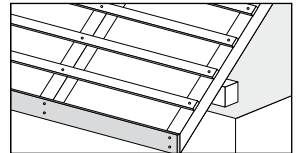
Roof trim
