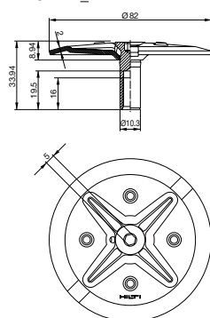
X-CRM8-15-12 P8
