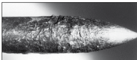
Mechanically cleaned point of a pulled-out DX fastener
