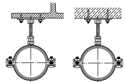
Hangers with threaded connectors
