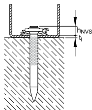
X-GN/GHP: h_{NVS} = 2-5 mm
