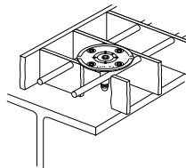
Grating fastenings
