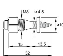
X-EM8H-15-12 FP10
