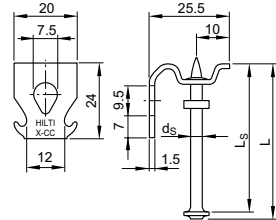
X-CC DKH 48 ③
