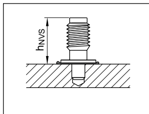
X-BT M8-15-6 SN12-R
