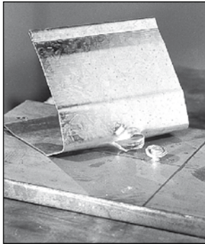
Sheet pull-over
