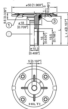
X-CRM8-15-12 FP10
