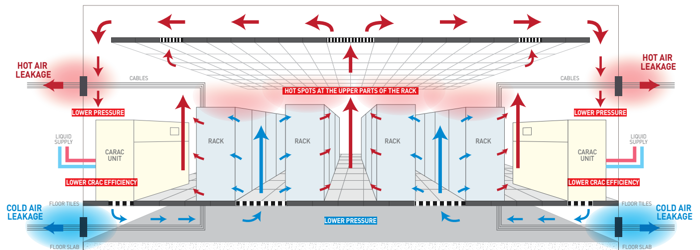
Fig. 1: Impact of penetration leakage on airflow in data centers with cold/hot aisle containment - Adapted from ASHRAE [6] [7]
