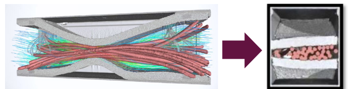
Fig. 8: Competitive pathway device with rubber band around intumescent liner pads to adjust to cable penetrants – third-party CFD simulation by Paul Scherrer Institute from June 2016
