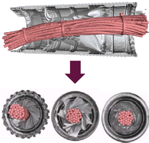
Fig. 6: Hilti Speed Sleeve CP 653 / CFS-SL with closing mechanism to increase air tightness – third-party CFD simulation by Paul Scherrer Institute from June 2016
