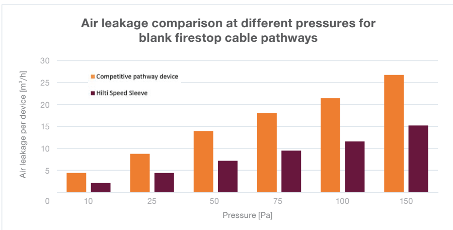
Fig. 3: Air leakage comparison for firestop cable devices at 40% fill acc. EN 1026 - third-party test reports from December 2016
